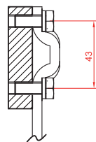
Mounting on yoke with plane surface
