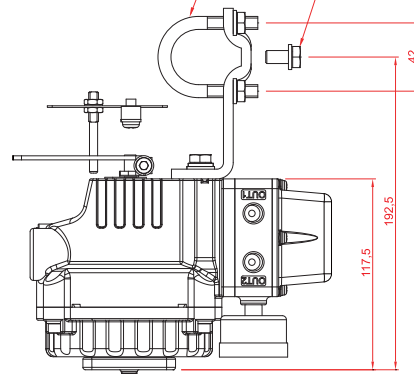
Mounting to linear actuators to IEC 60534 6-1
